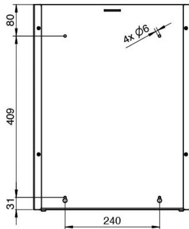
Bohrbild | drilling pattern
