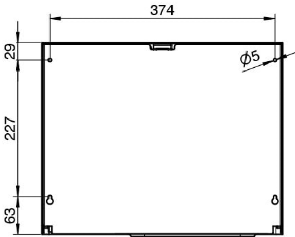
Bohrbild | drilling pattern
