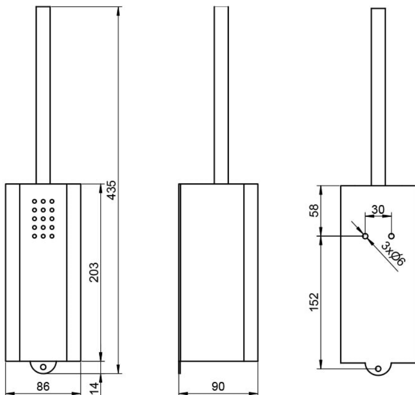
Bohrbild | drilling pattern
