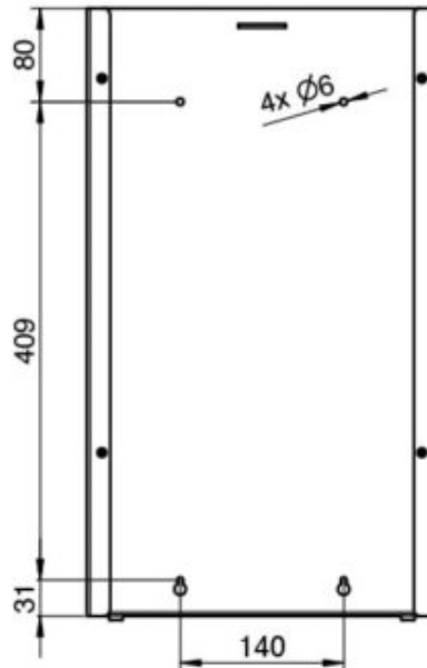
Bohrbild | drilling pattern
