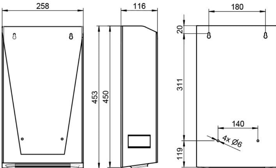
Bohrbild | drilling pattern
