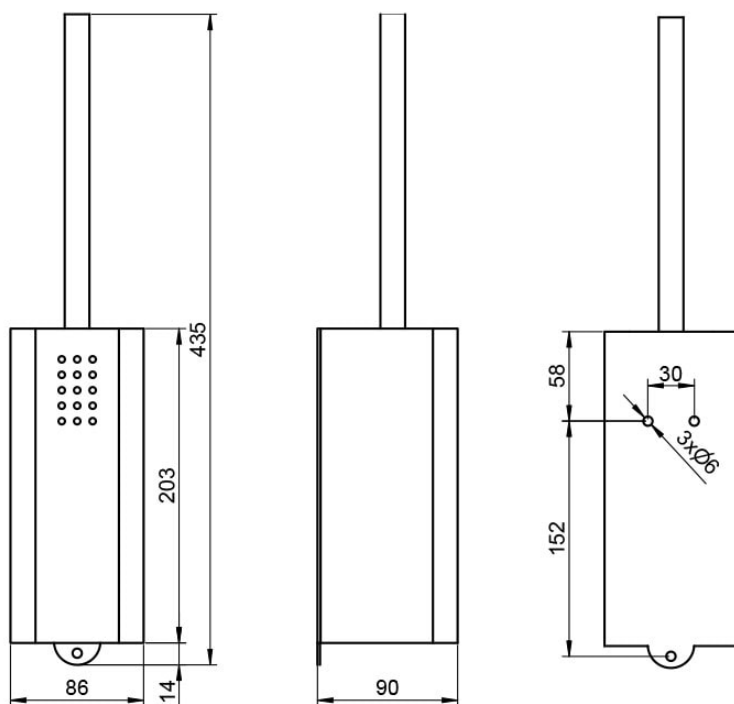
Bohrbild | drilling pattern
